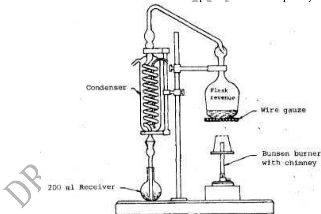
FIGURE 1 – Distillation Assemble
