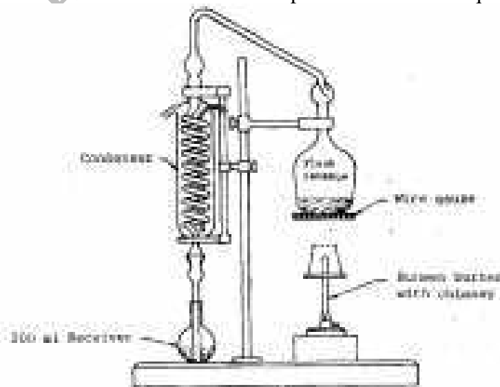
FIGURE 1 – Distillation Assemble
