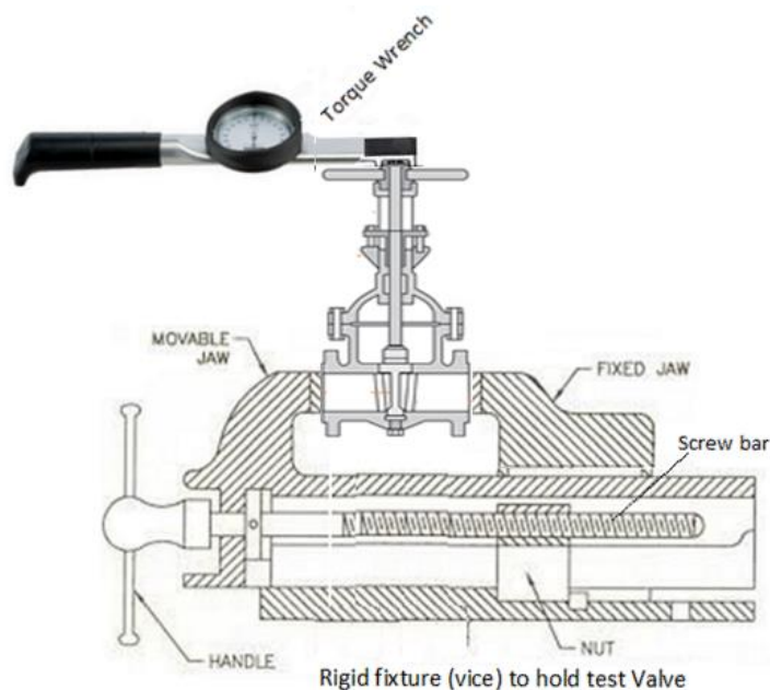
Figure 7- Test Apparatus for Test of operating load
