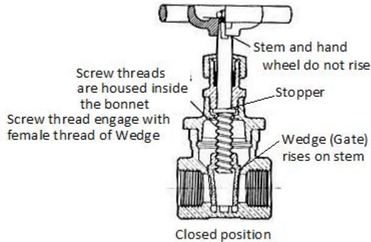
Figure 2C- Non-Rising Stem Inside Screw
