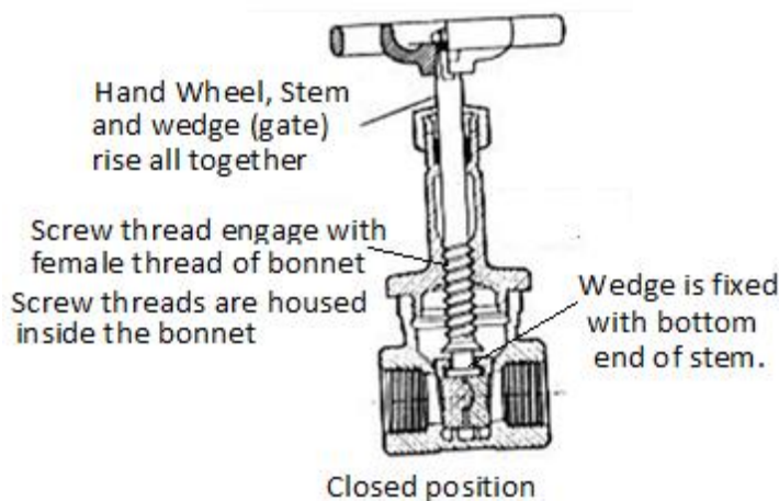
Figure 1C-Rising Stem Inside Screw
