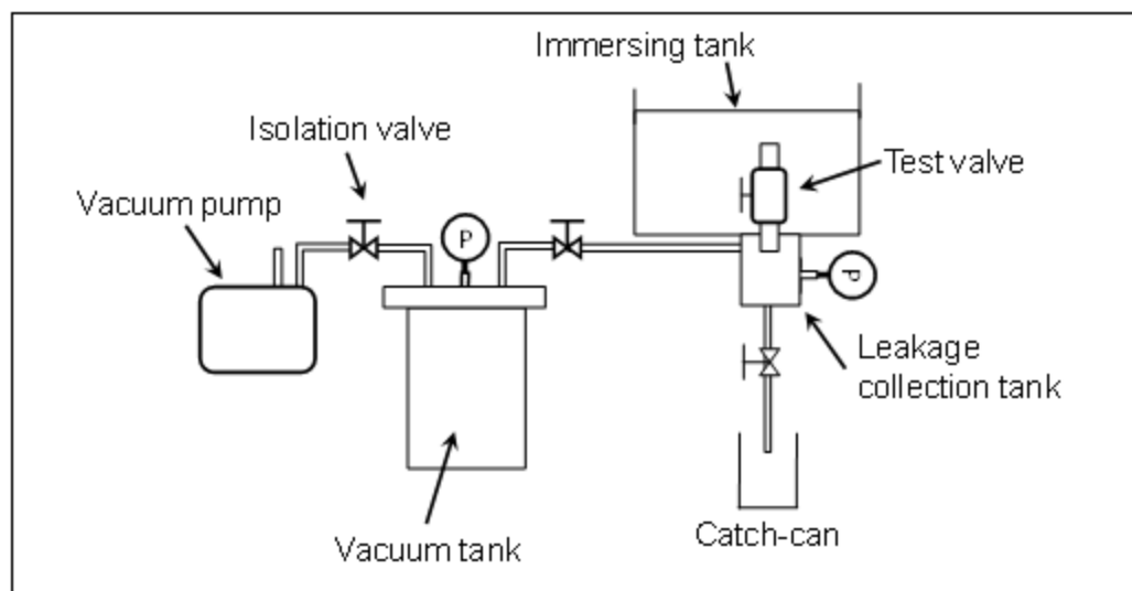
Figure 11-Vacuum test apparatus
