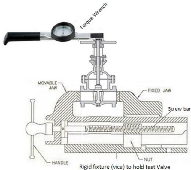
Figure 2- Apparatus for testing of operating load
