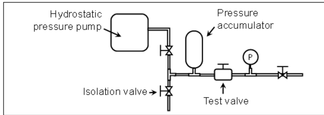
Figure 10- Hydrostatic pressure test apparatus
