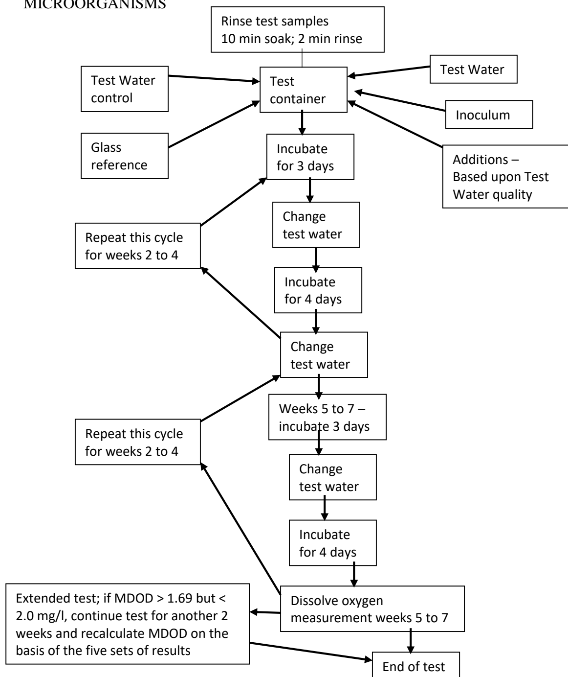
Fig. D-1: Flow diagram - the sequence of the test procedure GROWTH OF AQUATIC MICROORGANISMS
