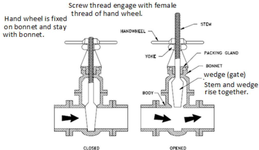
Figure 3C- Outside screw and yoke (OS&Y)- Rising Stem
