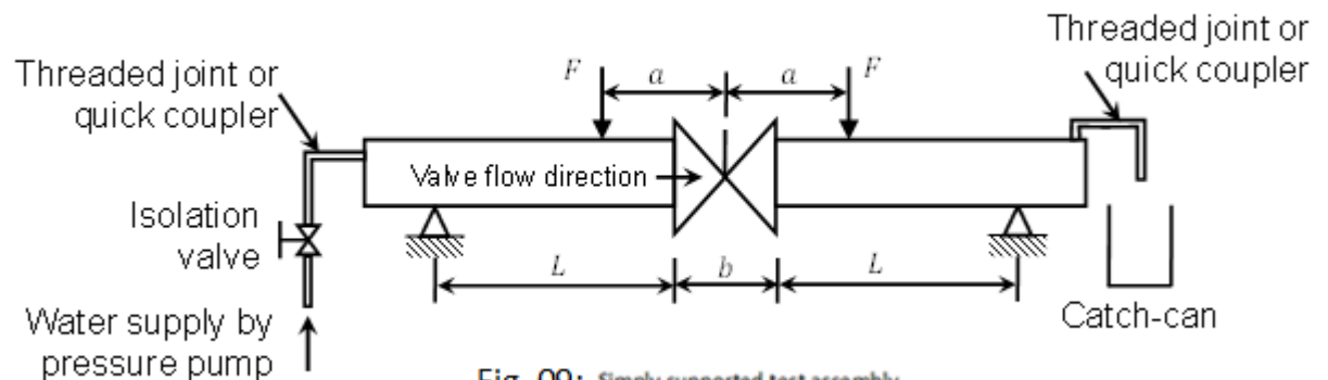
Fig. 09: Simply supported test assembly
