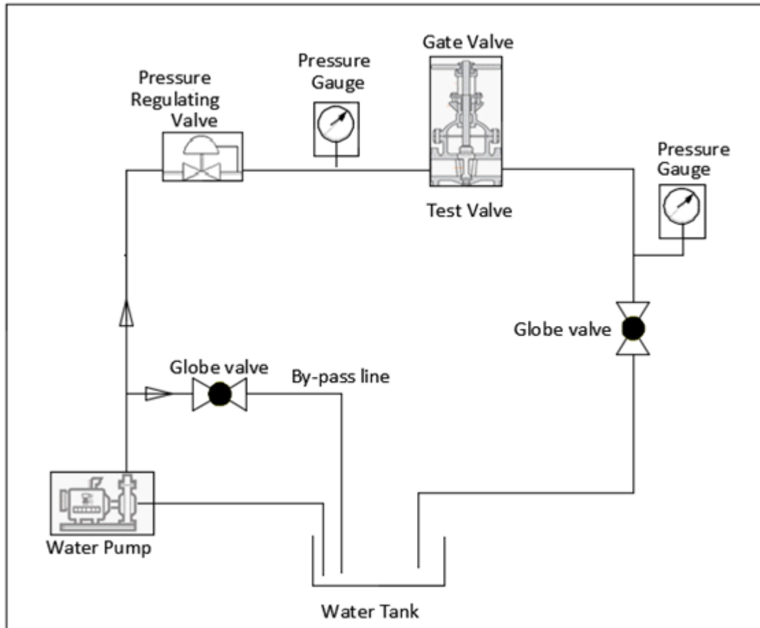
Figure 5- Test Apparatus of Test of resistance to internal pressure
