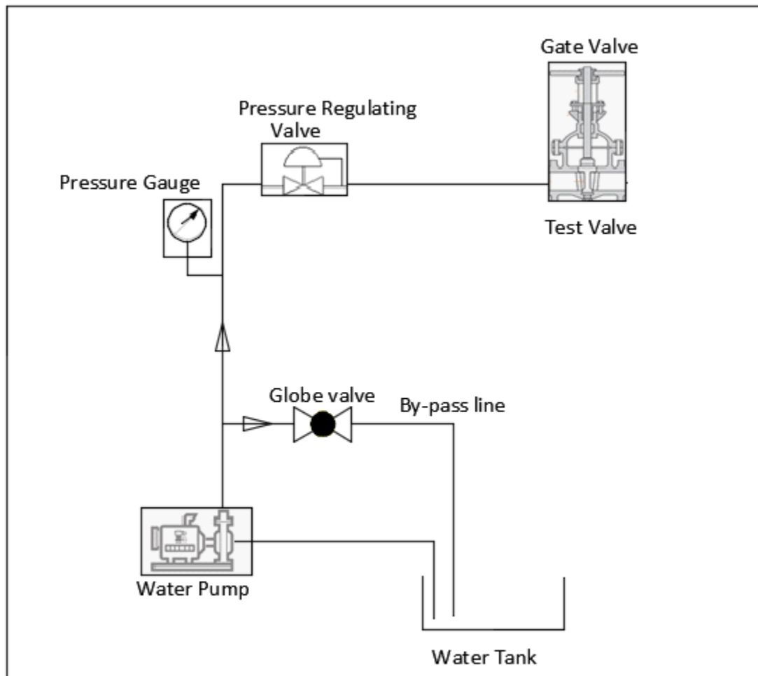
Figure 6- Test Apparatus of Test of resistance to internal pressure
